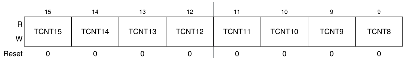
Figure 22-10. Timer Count Register High (TCNTH)
