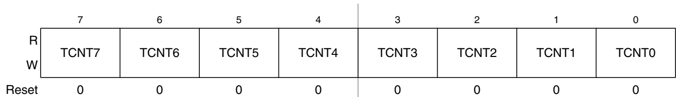
Figure 22-11. Timer Count Register Low (TCNTL)
